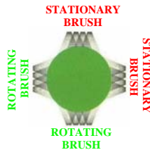
Section view-4 brushes
